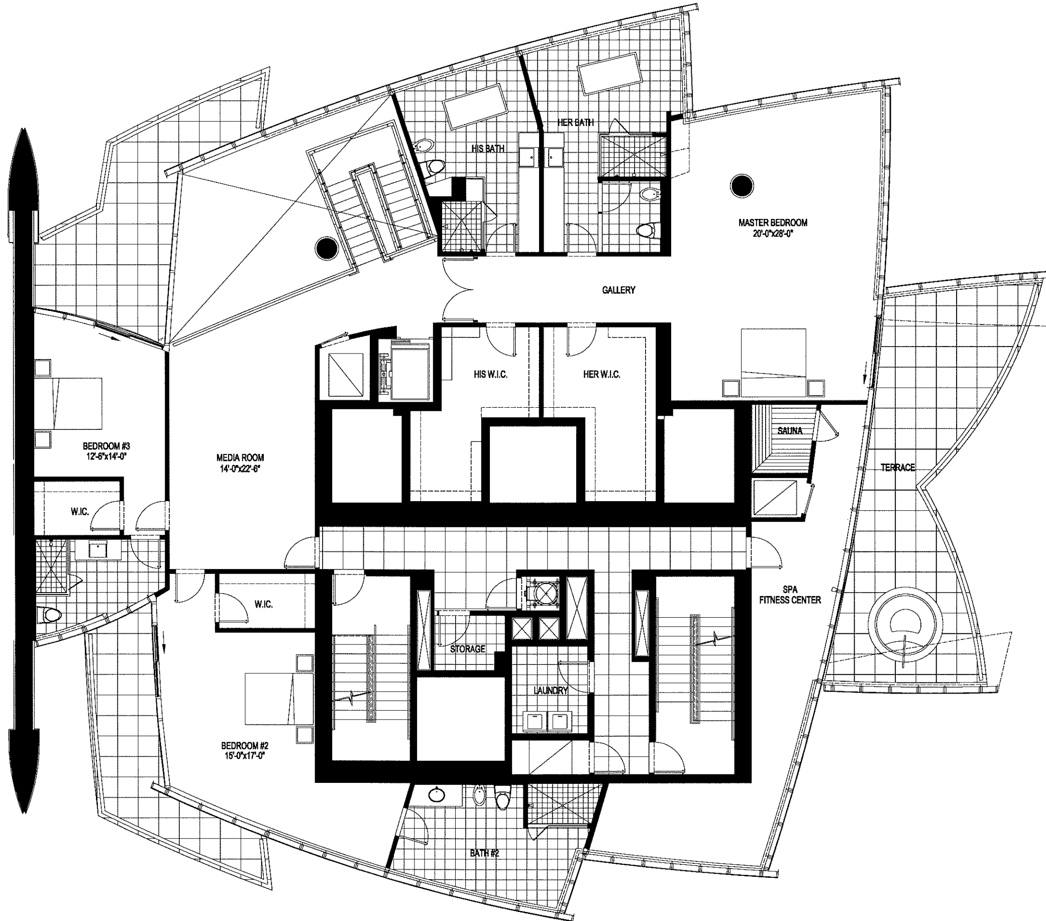
PENT HOUSE I LEVEL 2
